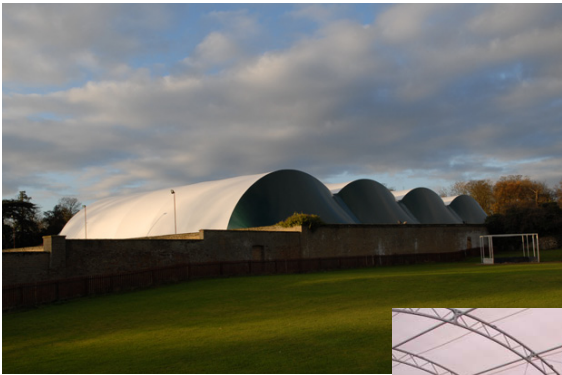
CULFORD SCHOOL 4 no. 18m wide x 37.5m long x internal height 9.2m
